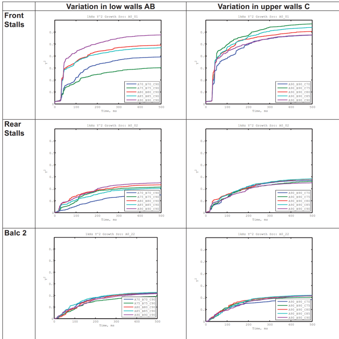
Figure 6. Growth of lateral energy Y across different room geometries. 30msec window, 2ms step. 1kHz octave band. Vertical scale is arbitrary, but equal across all figures, not normalised to W.
